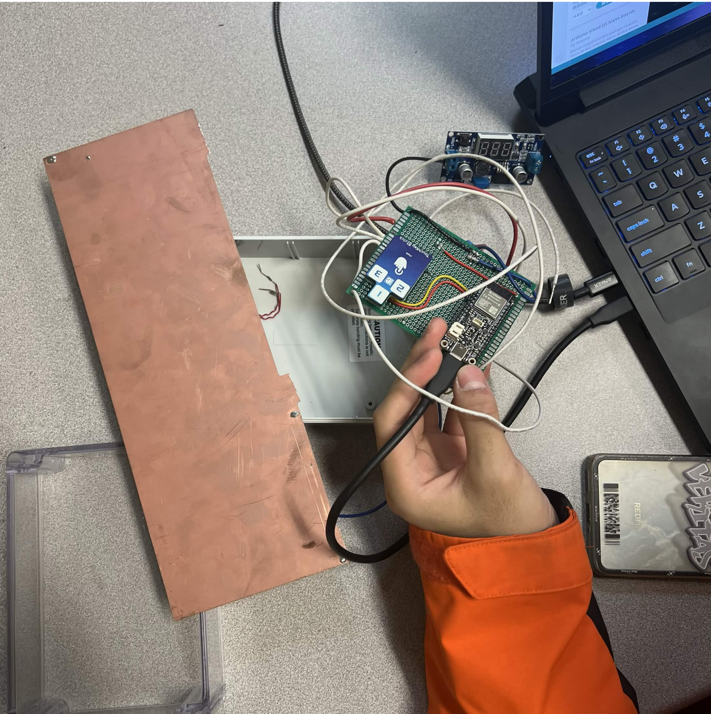
ESP32 + LM2596 buck + optocoupler module wired to PLC X7.
